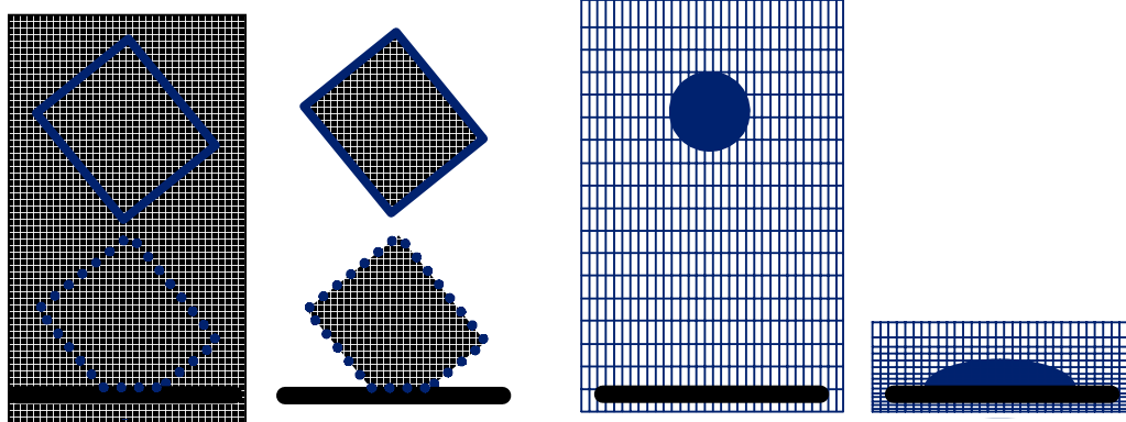
Sl. 6. Uporaba PLE opisa Fig. 6. Applications of the ALE formulation
