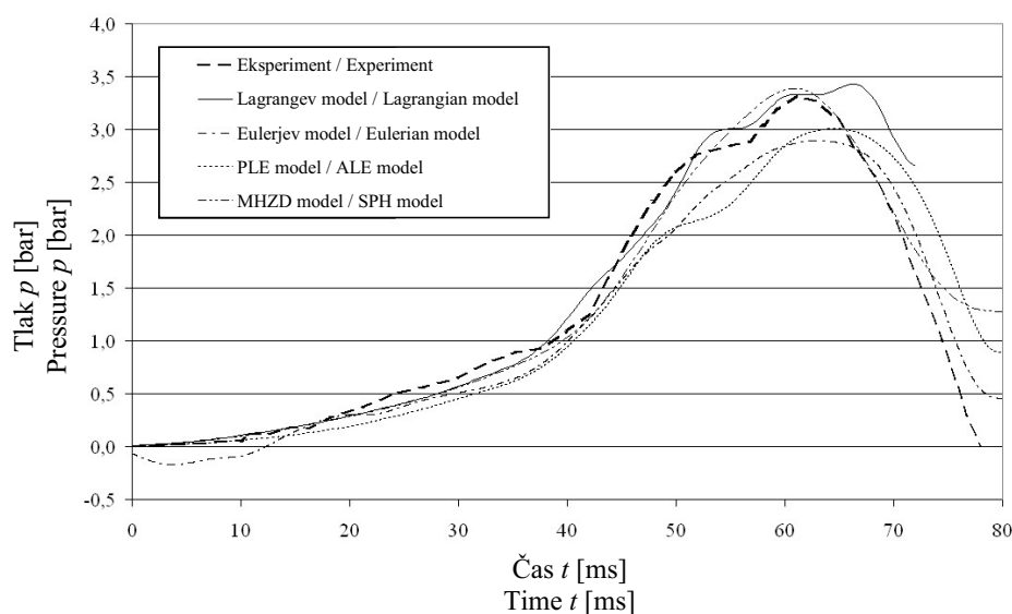
Sl. 11. Primerjava časovne spremembe tlaka v točki 1 Fig. 11. Comparison of the pressure time-variation at point 1
