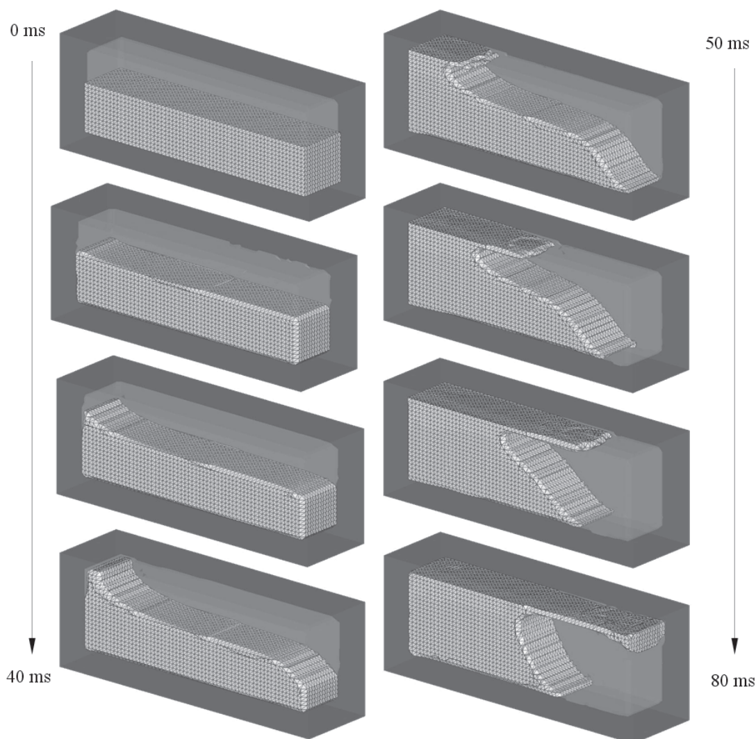
Sl. 10. Gibanje tekočine, modelirane s PLE opisom Fig. 10. Fluid motion modelled with ALE formulation
