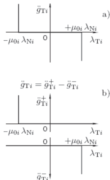
Sl. 3. Dopolnilnost v tangentialni smeri Fig. 3. Complementarity in the tangential direction
